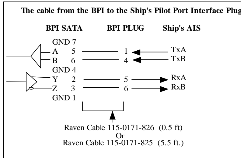
Figure 4 – BPI Cable Wiring Diagram
