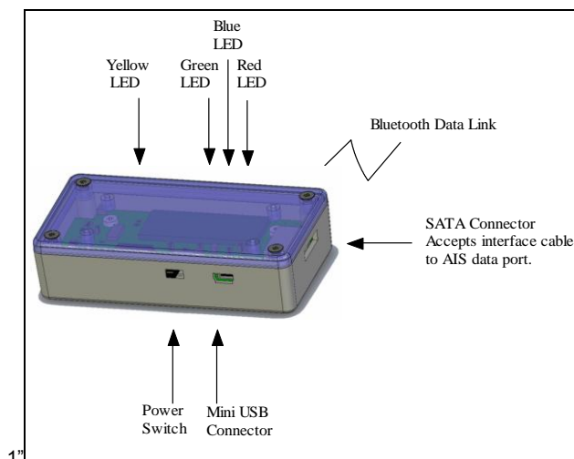
Figure 2 - Overview of the BPI
